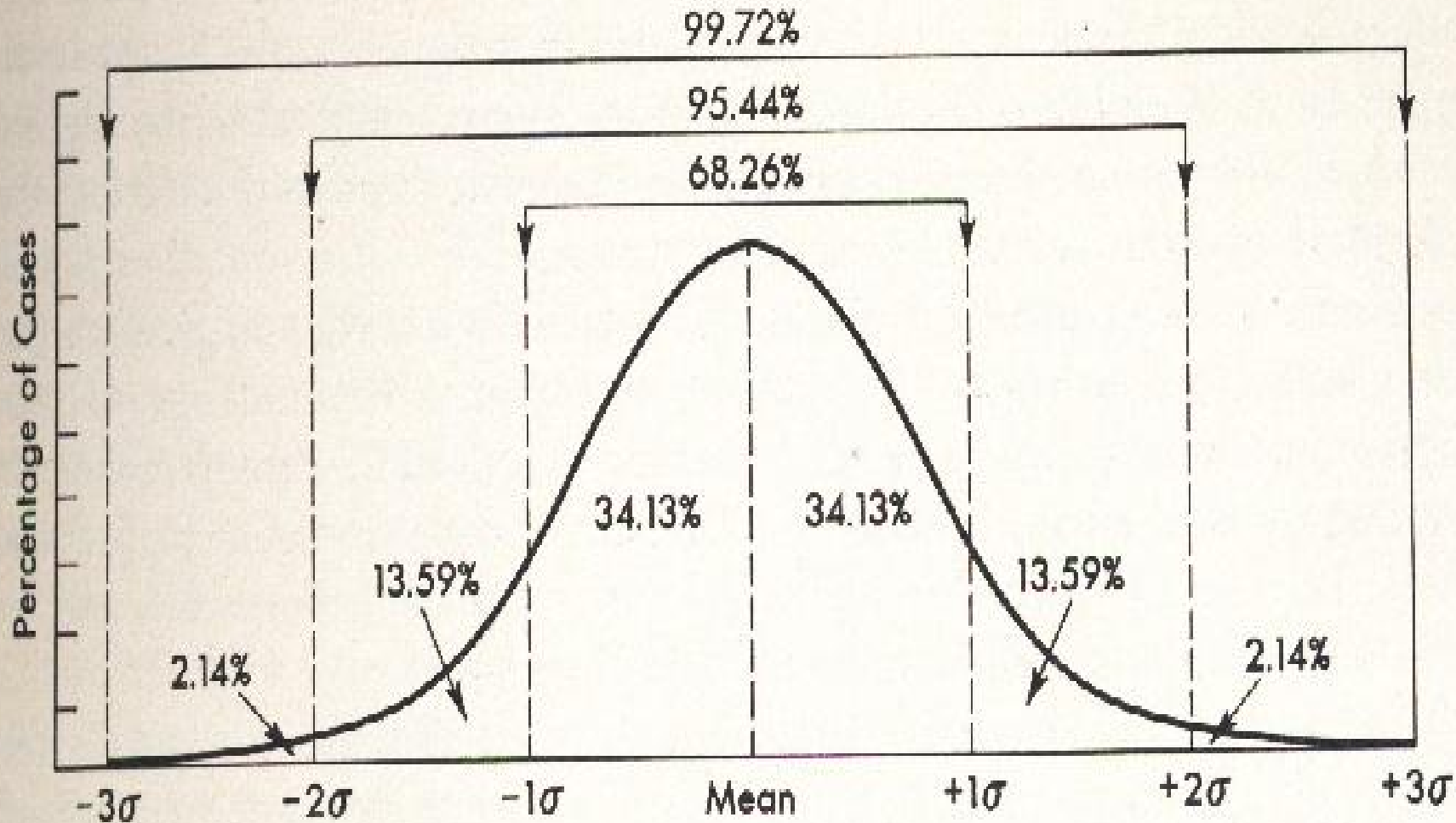
FIG. 3. Percentage Distribution of Cases in a Normal Curve.
